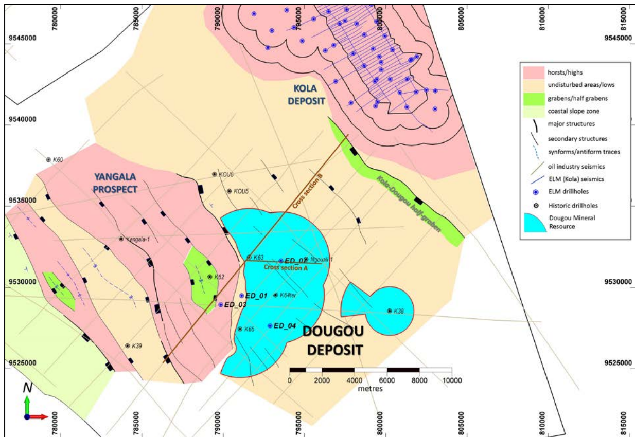
Figure 2. Simplified structural map locating the Dougou Carnallite Deposit along with the Kola Sylvinite Deposit and Yangala Sylvinite Prospect. Section lines for A (Fig. 3) and B (Fig. 4) are drawn.
